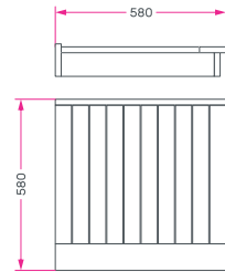
Sauna bench model CHALEUR DE LUXE in Ayous, price per running meter - 585mm
