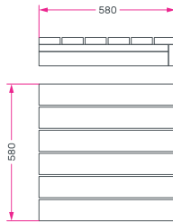
Sauna bench CHALEUR PRO in Ayous 28x90 (price/r.m.)
