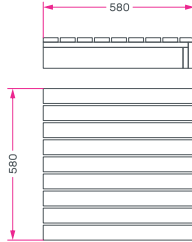
Sauna bench CHALEUR Private in Ayous 17x57 (price/r.m.)
