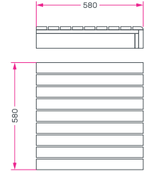
Sauna bench CHALEUR Private in Thermo-Ayous
