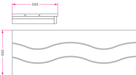
Sauna bench model Wave in solid Ayous, price per running meter - 585mm
