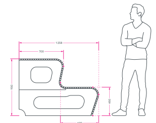
Sauna luxury bench in Ayous/Cedar wood, price/r.m
