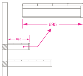
Sauna cantilever bench in solid ayous or cedar 175mm wide, price per running meter 695mm
