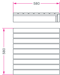
Sauna bench CHALEUR Private in Cedar (price/r.m.)
