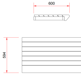
Sauna bench NEW CHALEUR, Ayous
